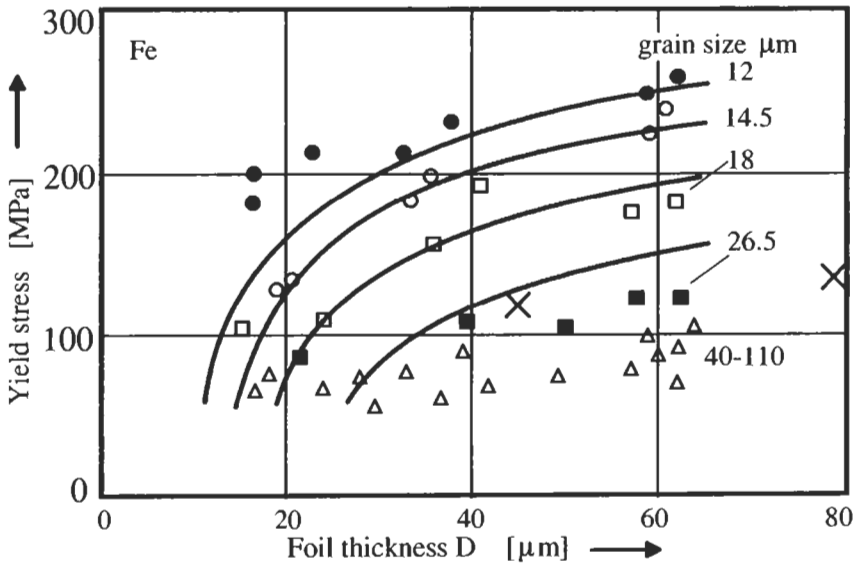
Fig. 28. Dependence of the yield stress on grain size and sample thickness in thin Fe ribbons (Judelewicz, 1993). For an explanation of the fitted curves see text. The 2 measurements marked with x were obtained by Miyazaki et al. (1979) for a grain size of 25 μm.
