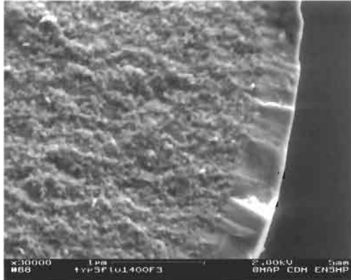
Fig. 15. The surface of a Hi-Nicalon Type S fibre showing the layer of silica which has formed during creep at 1400°C.
