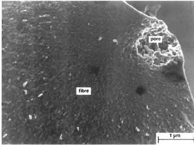
Fig. 14. Local inhomogeneities can lead to degradation at the surface of the fibres when heated above 1200°C in air, as in this Hi-Nicalon fibre.
