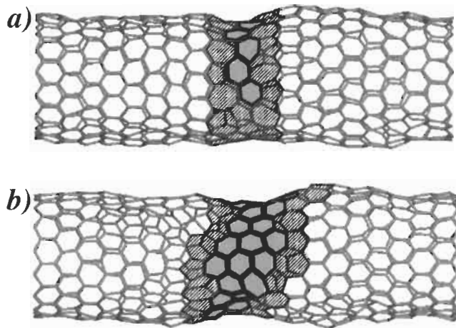
Fig. 11. Time evolution of the (17,0) tube with an addimer under 7.5% strain at 3000 K, illustrating the spontaneous winding of the defect about the tube: (a) initial configuration consisting of a single turn; (b) final configuration corresponding to about 3 turns after 1 ns.
